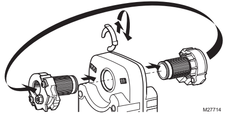
Fig. 7. SCSA Mounting
