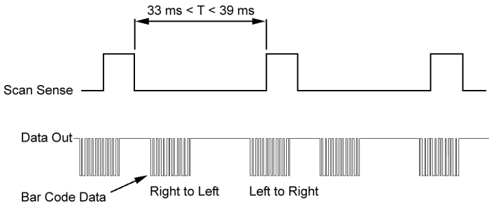
Figure 12: Timing Diagram
