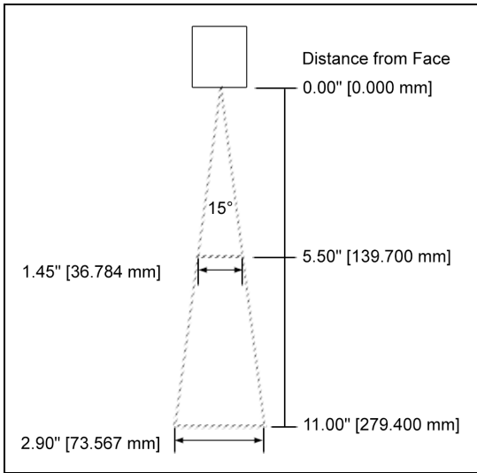
Figure 5. IS4125 Object Detection Field
