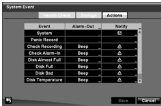
Figure 3-79 System Event Actions Screen
