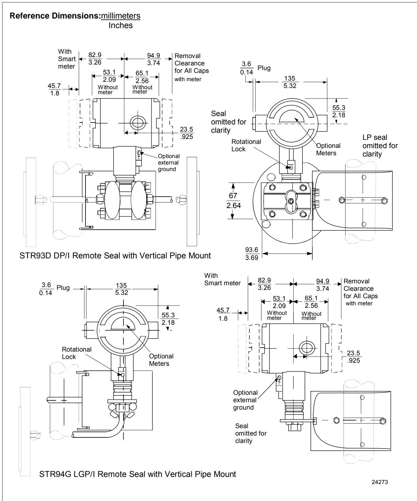
Figure 20 —Approximate vertical mounting dimensions for Remote Seal Transmitter
