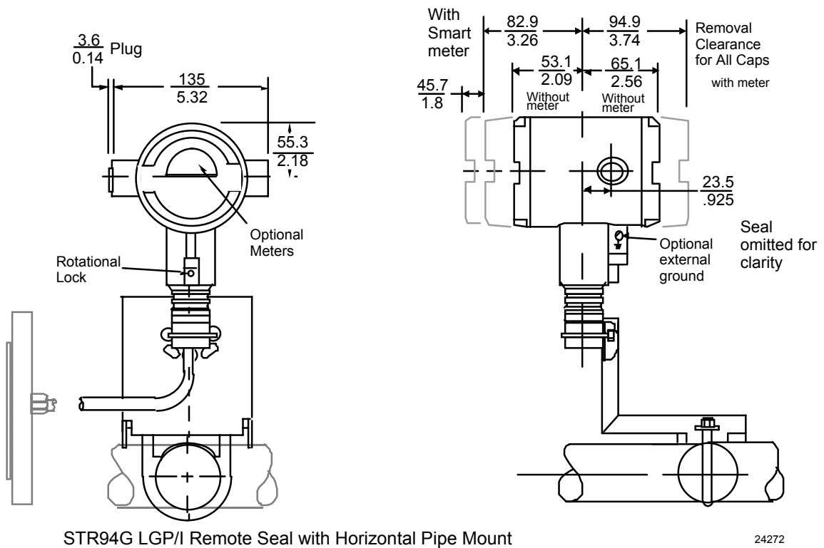
Figure 19 —Approximate horizontal mounting dimensions for Remote Seal Transmitter.
