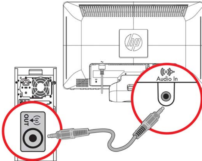
Figure 3-10 Connecting the audio cables - connector locations may vary
