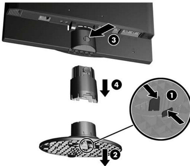
Figure 2-2 Removing the Monitor Center Column and Base
