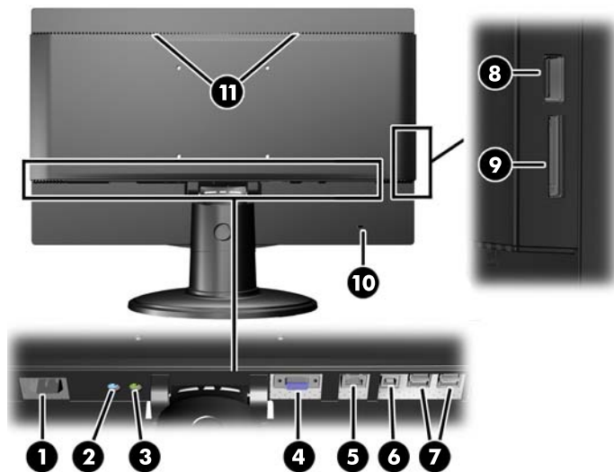
Figure 2-5 Rear Components
