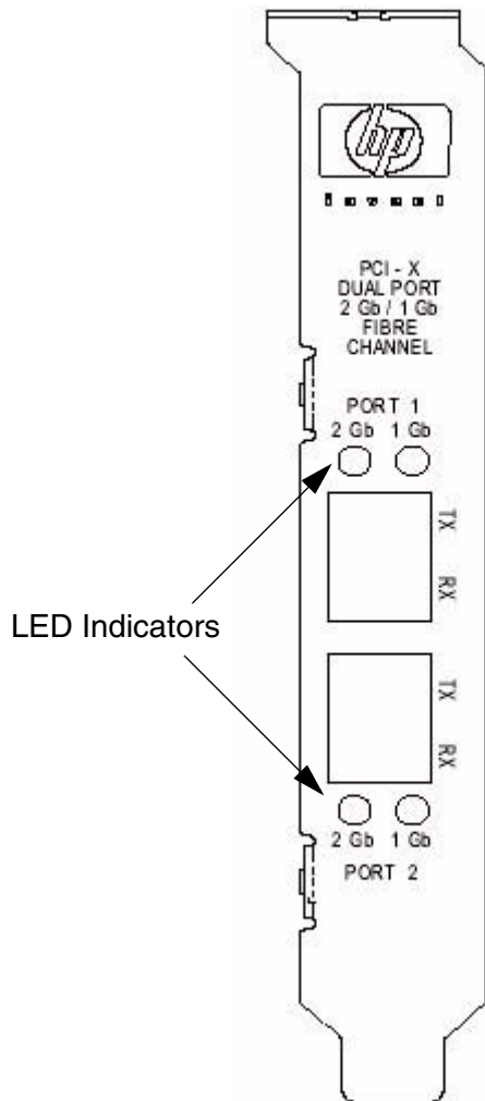
Figure 1 A6826A components
