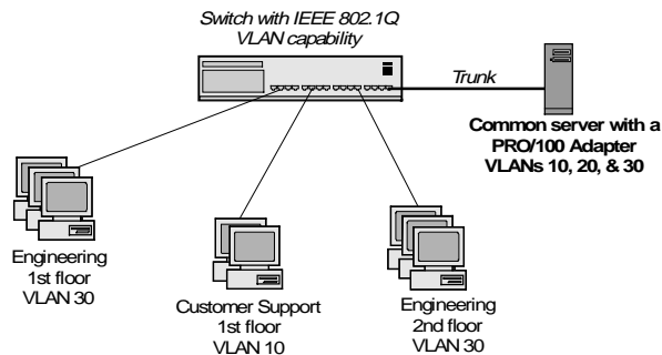
Figure 7-1. Virtual LAN Configuration
