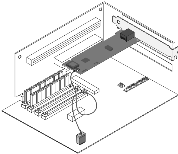
Figure 4-1. Connecting the Wake On LAN Cable
