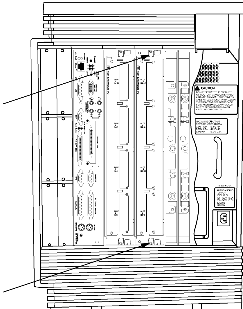
Figure 2 Screw Locations
