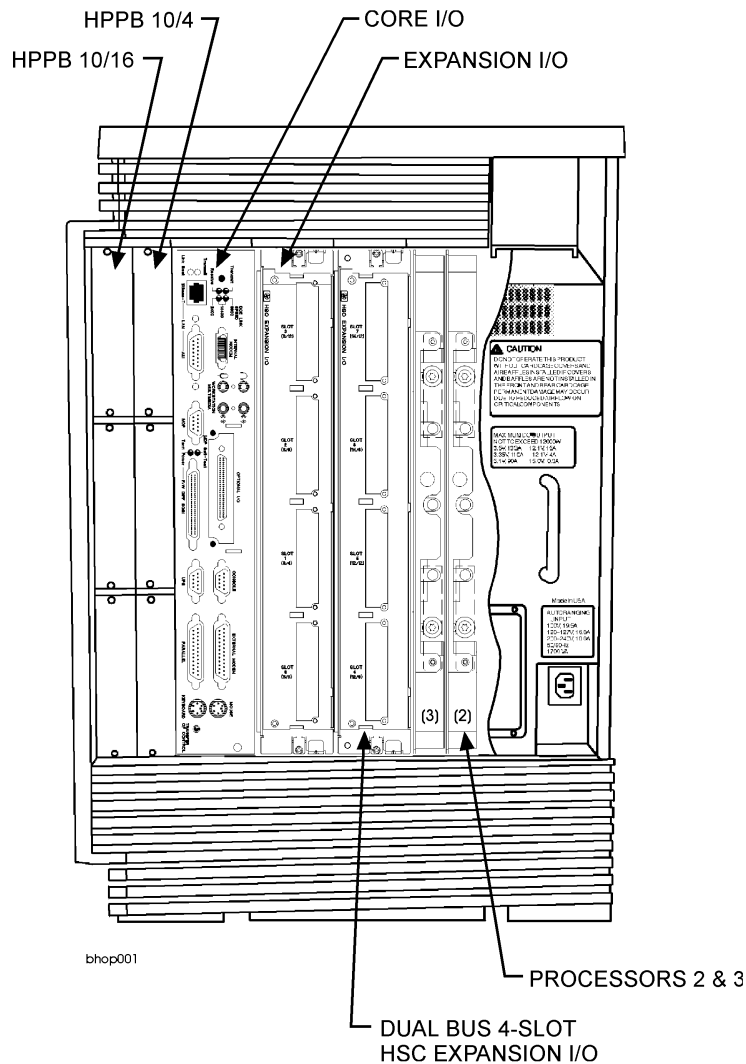
Figure 1 HP9000/K570 Rear View
