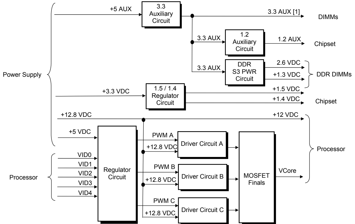
Figure 7-4. Low Voltage Supply and Distribution Diagram
