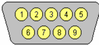
Figure 5-3. Serial Interface Connector (Male DB-9 as viewed from rear of chassis)
