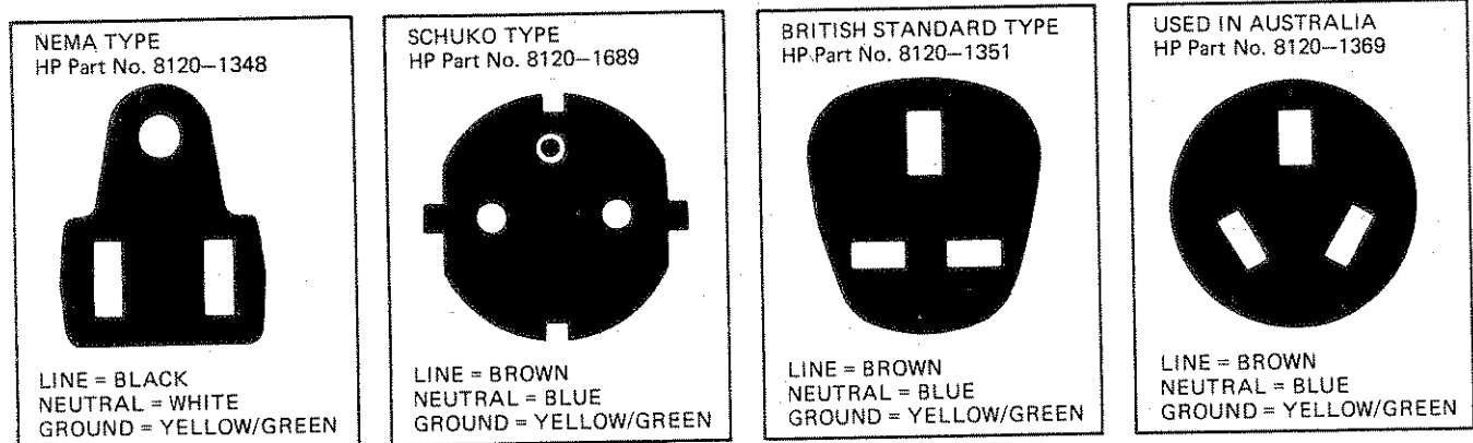
Figure 2-3. Power Cords
