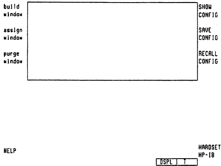
Figure 2-27. Select Window #1
