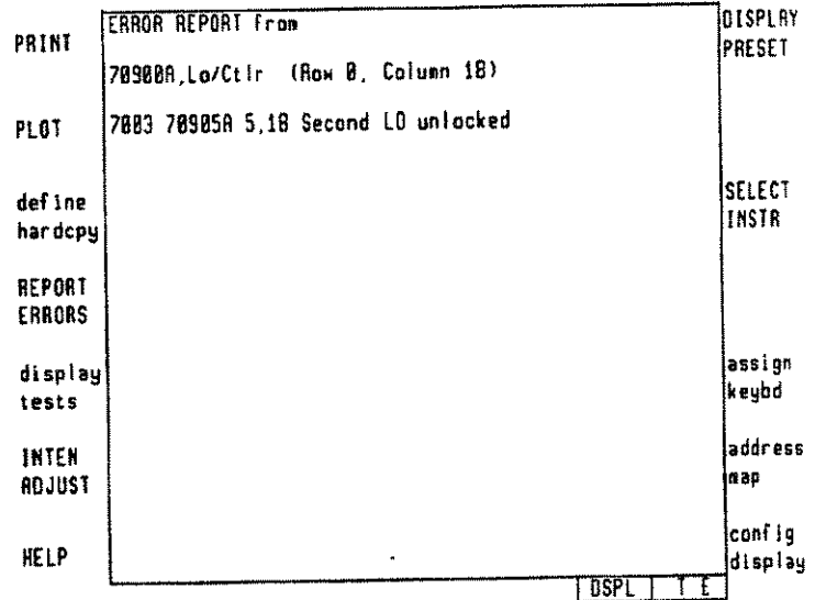
Figure 1-10. Report Errors
