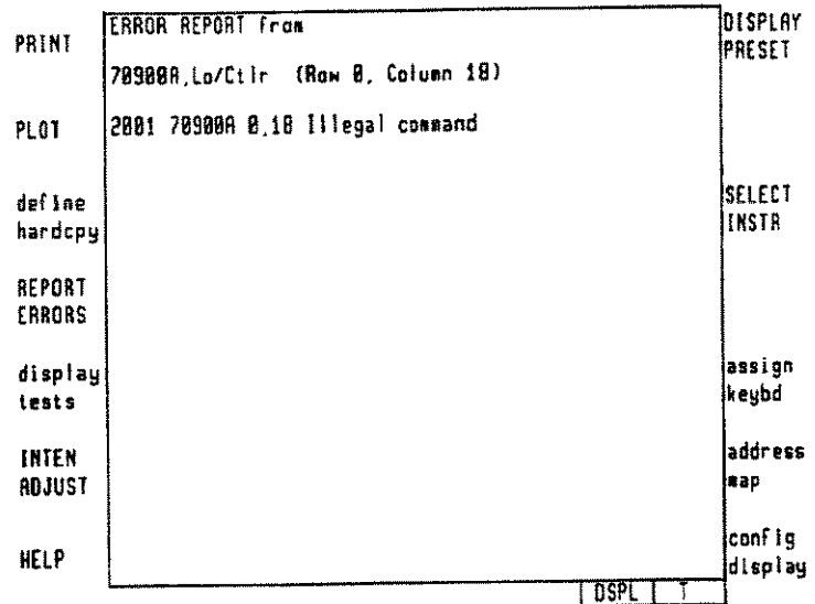
Figure 2-58. Reporting Errors
