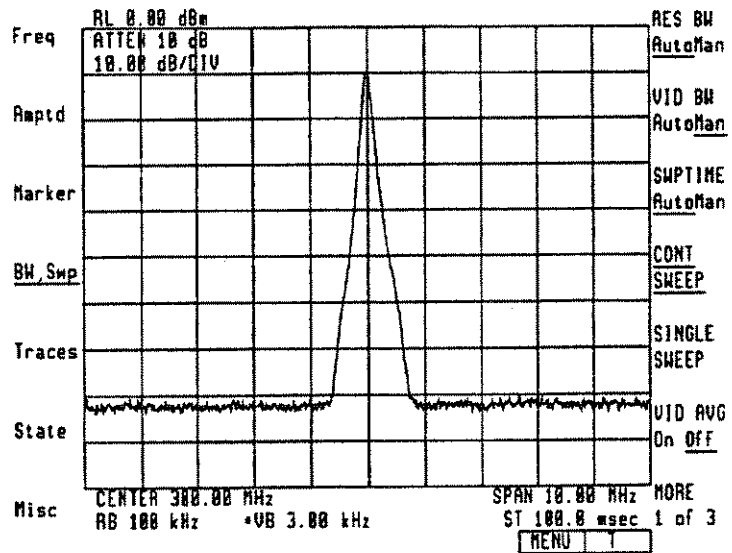
Figure 2-52. Plot Output
