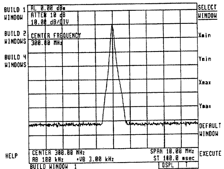
Figure 2-17. Build Window #1
