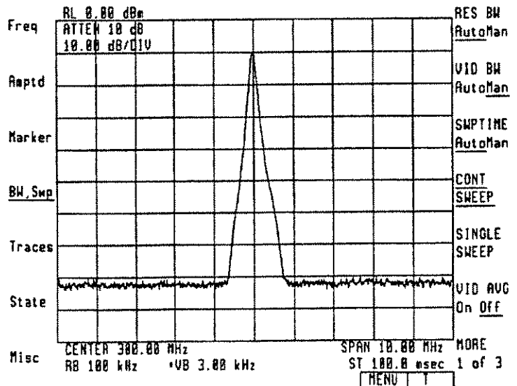
Figure 2-47. Standard Plot
