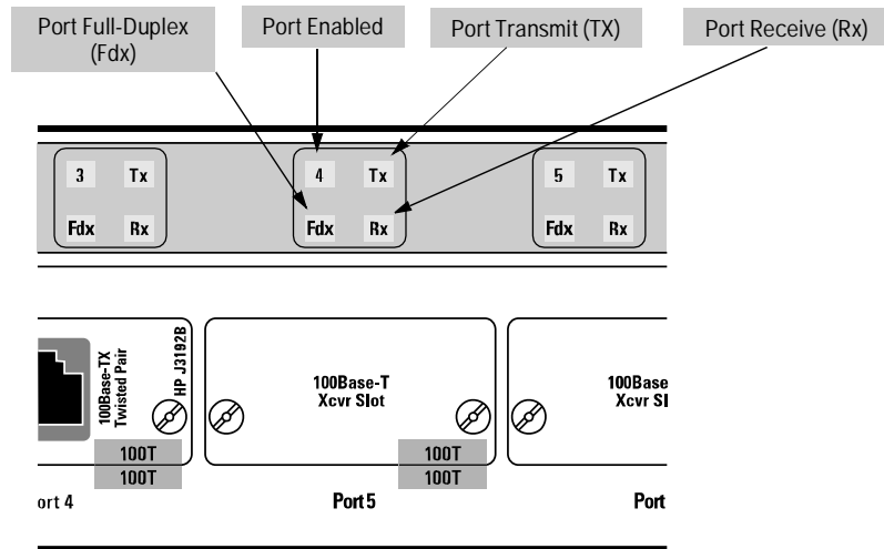
Figure D-2. Example of Port Status LEDs for the Switch 800T
