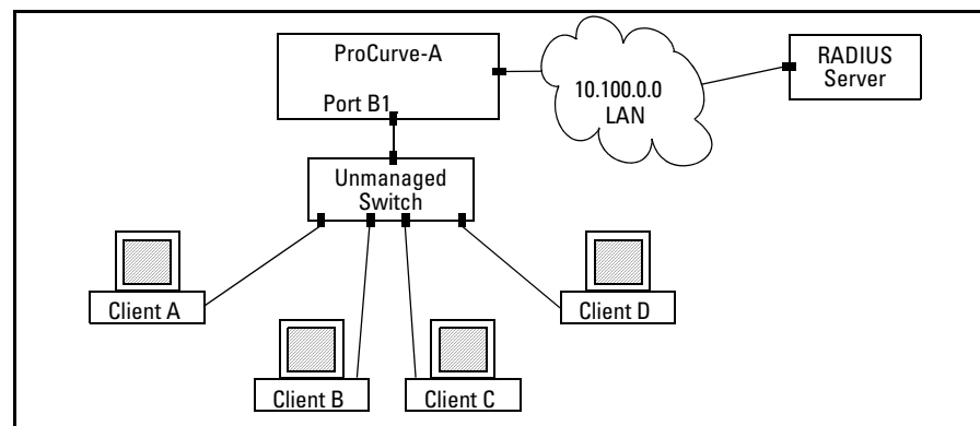
Figure 9-1. Example of Multiple Clients Authenticating Through a Single Port
