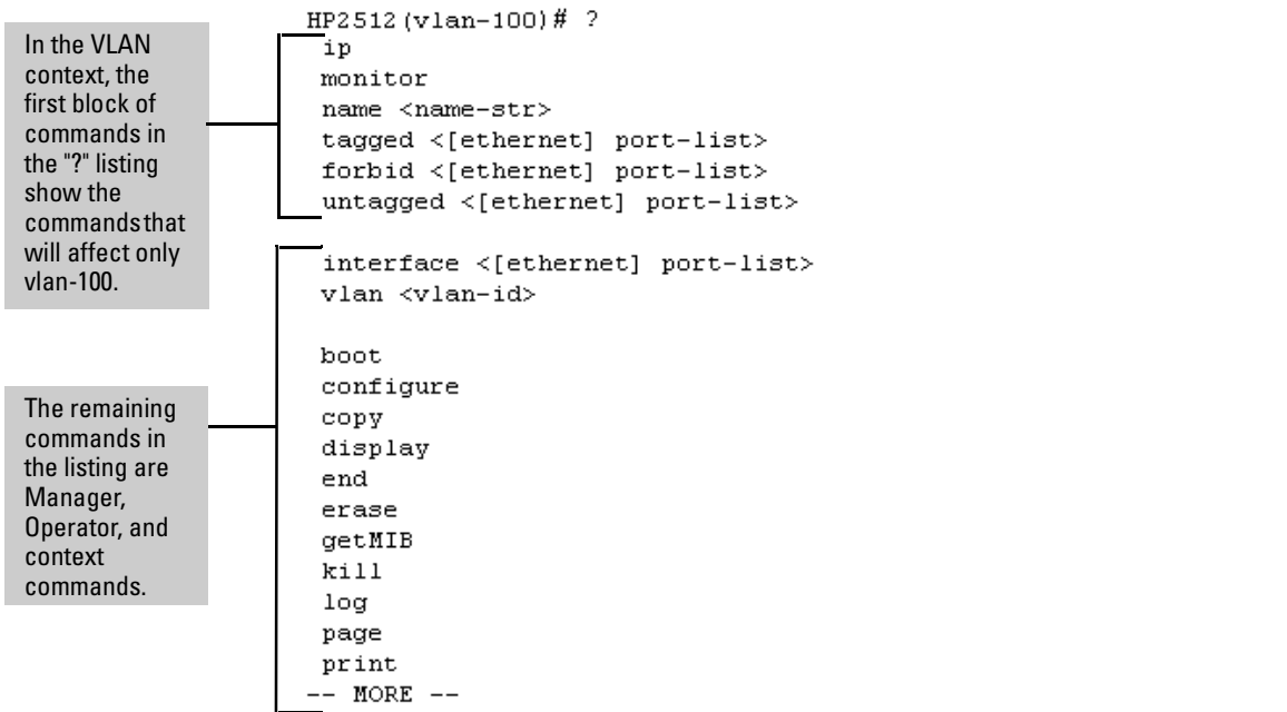
Figure 3-11. Context-Specific Commands Affecting VLAN Context
