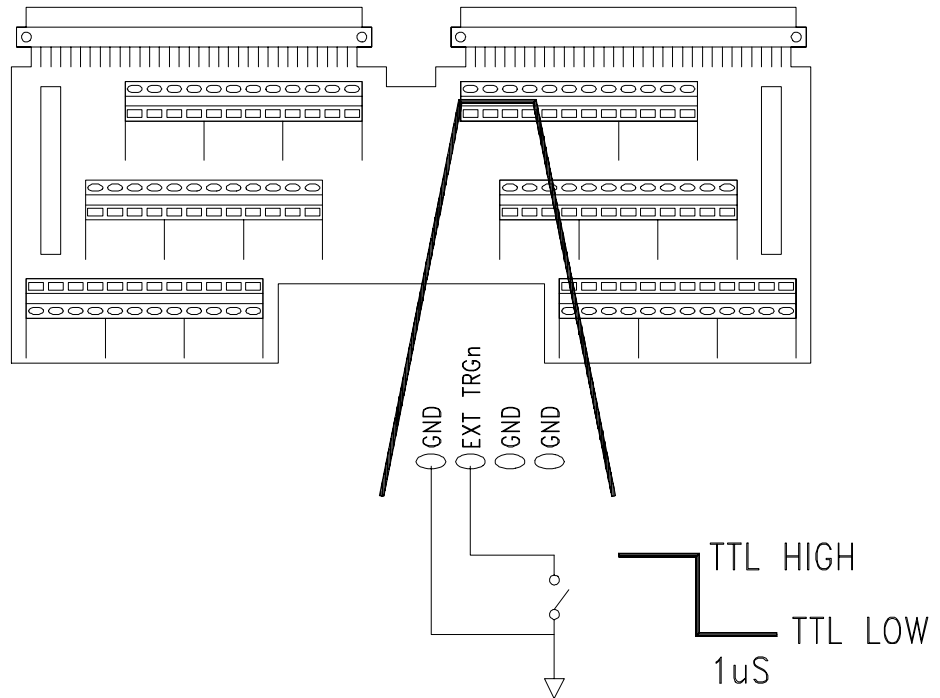
Figure 1-16. External Trigger Connections
