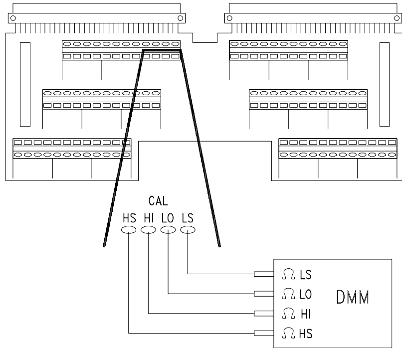
Figure 1-17. Calbus Connections
