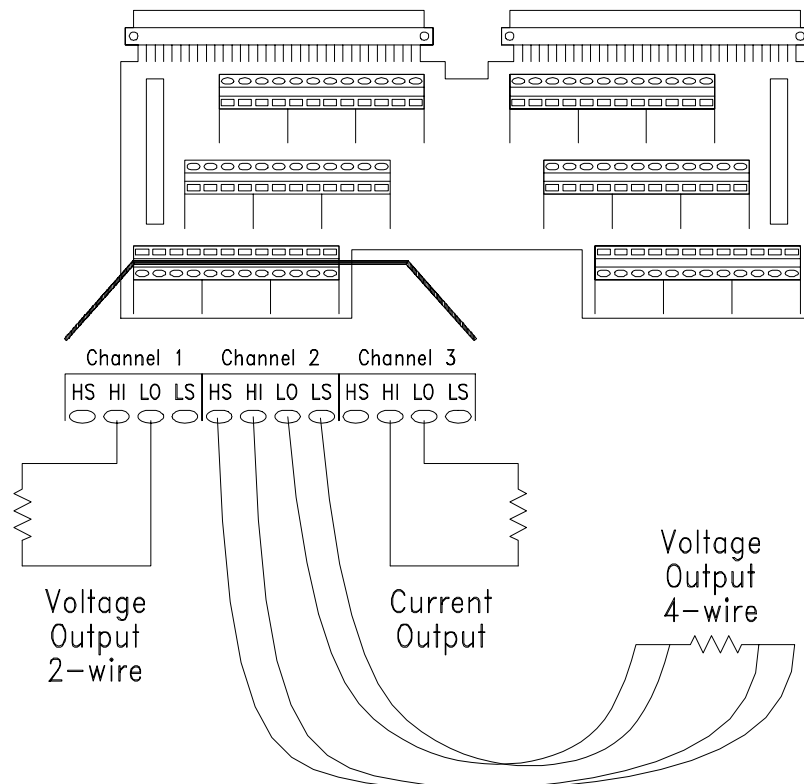
Figure 1-14. Typical Output Connections
