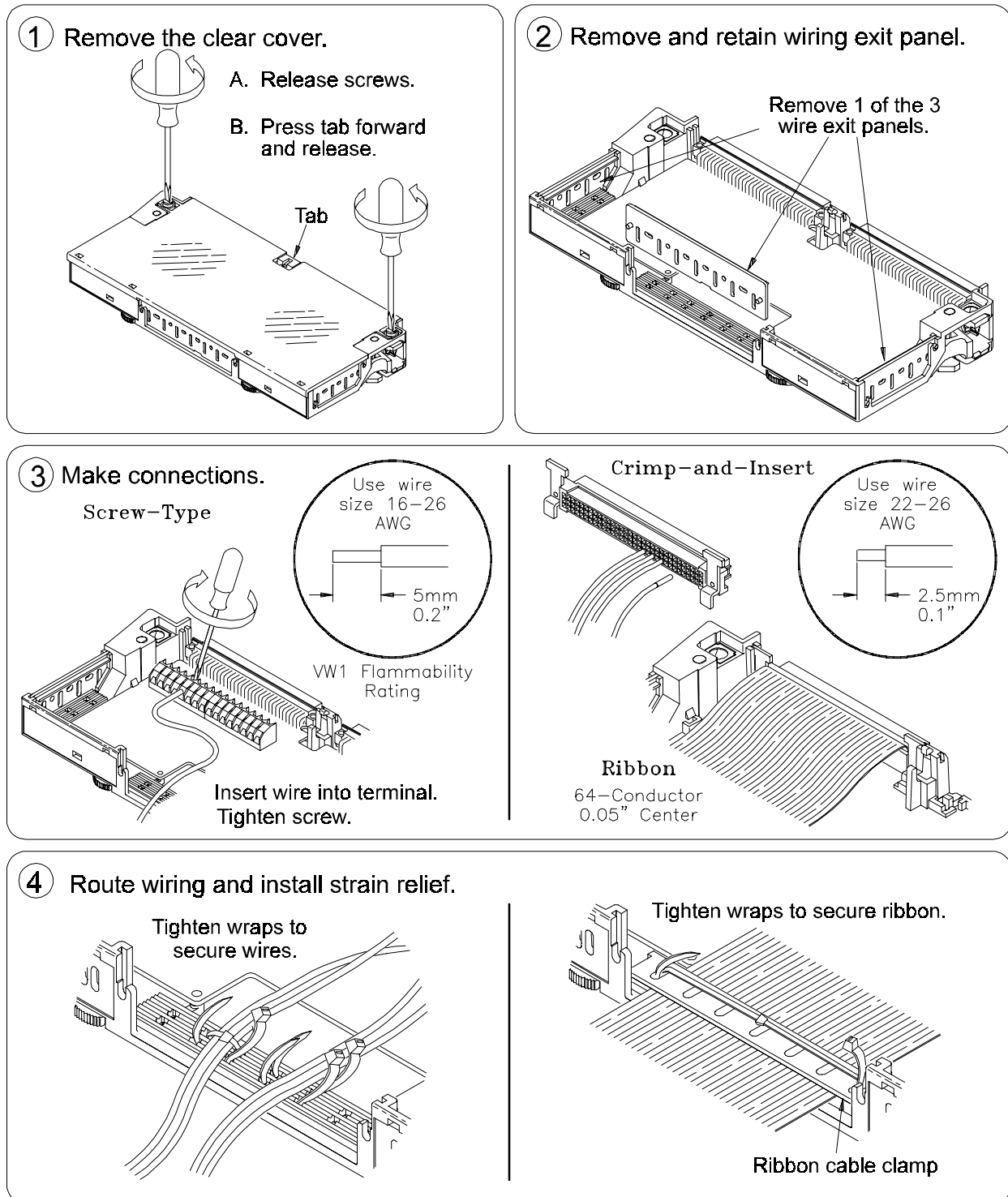
Figure 1-7. Wiring the HP E1418A Terminal Module (continued on next page)
