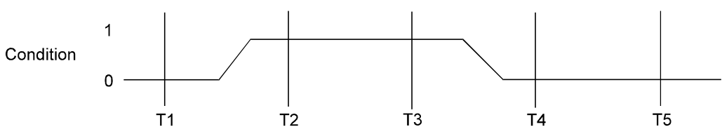
Figure 2-2. Typical Status Bit Changes in a Status Register
