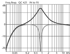
The figure above shows the HIGH MID EQ's curve when boosting (top curve) and cutting (bottom curve) frequencies.
