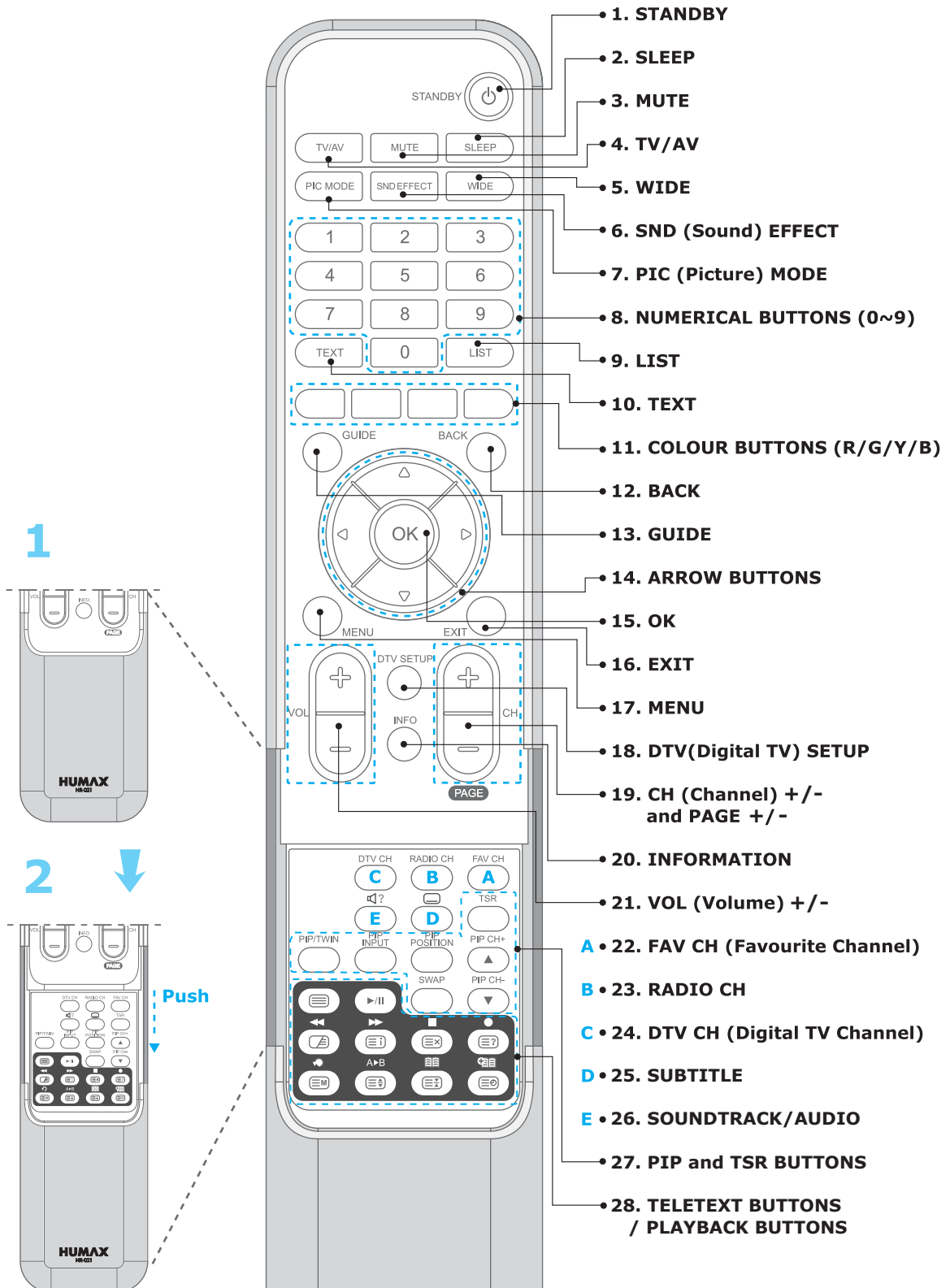
10. Remote Control
