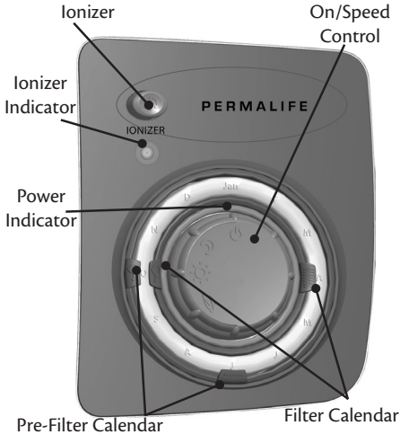
Figure 1 - Purifier Controls
