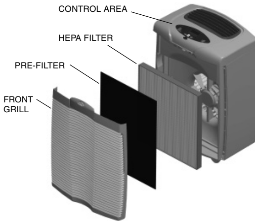
Fig. 2 - Air Purifier Components
