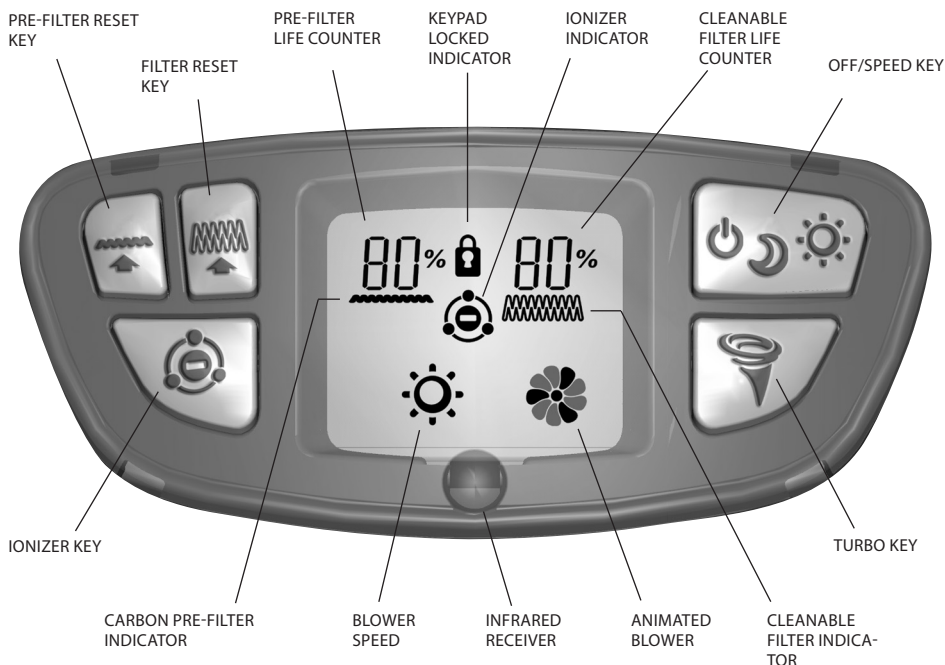
Fig. 3 - Air Purifier Control Area and Alpha-numeric Display
