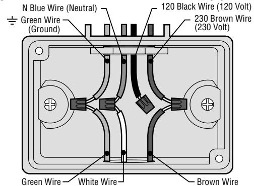
Figure 2 – Junction Box without Terminal Strip (230 Volt)
