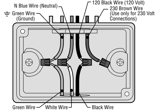
Figure 2 – Junction Box without Terminal Strip (230 Volt)
