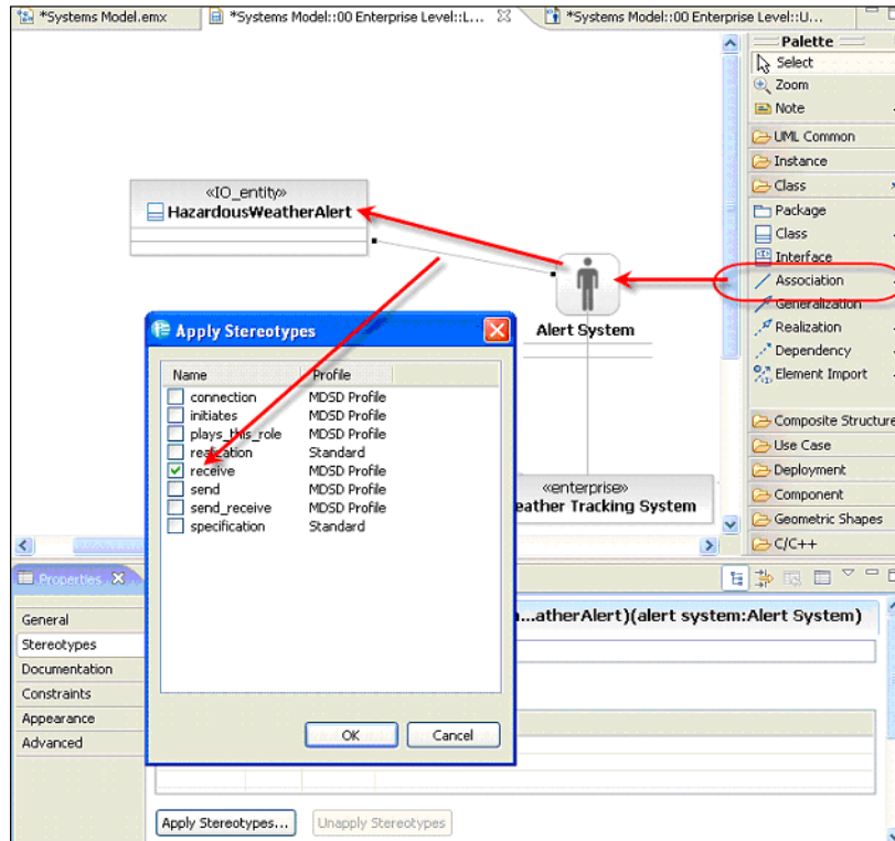
Figure 6-42 Creating associations with I/O entities
